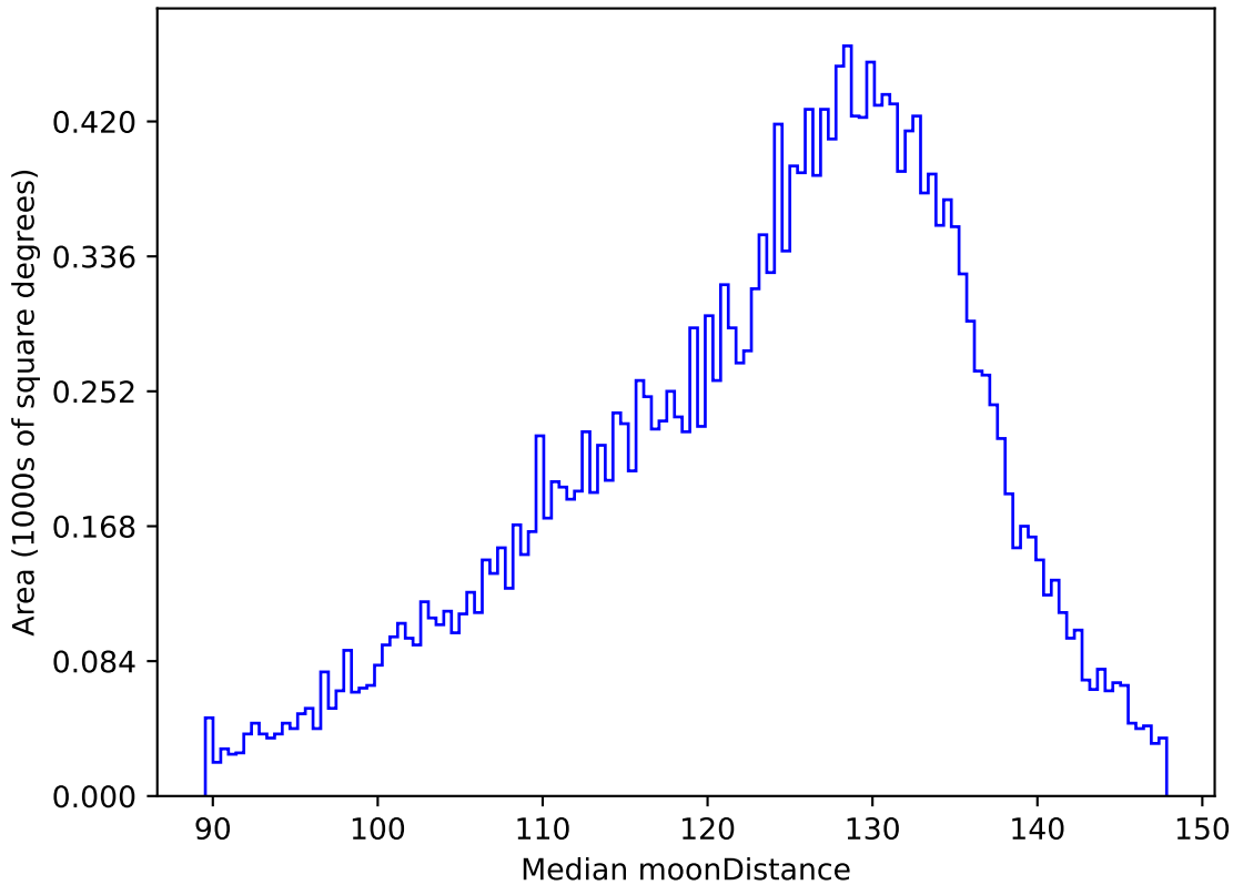
weather_cloudso14v3.4_10yrs All sky u band: Median moonDistance
