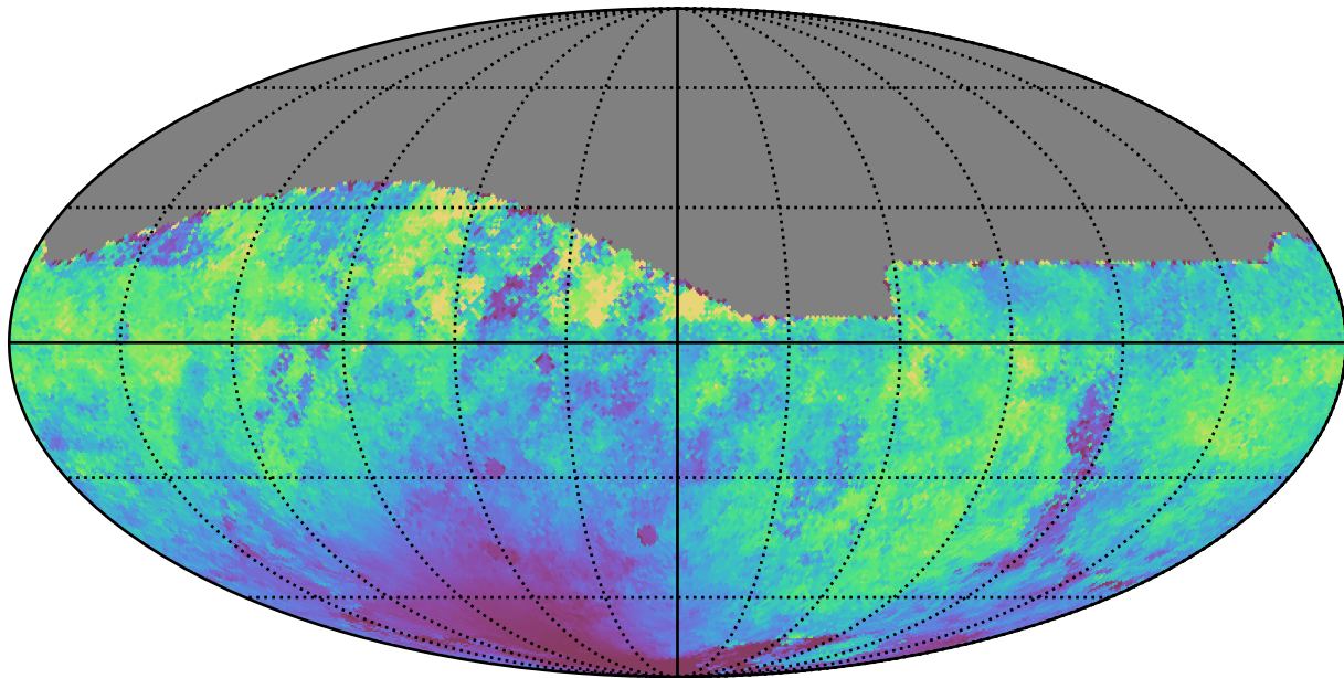
weather_cloudso14v3.4_10yrs All sky r band: Median moonDistance
