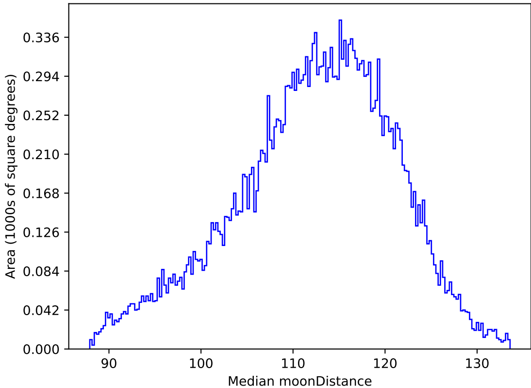
weather_cloudso14v3.4_10yrs All sky r band: Median moonDistance
