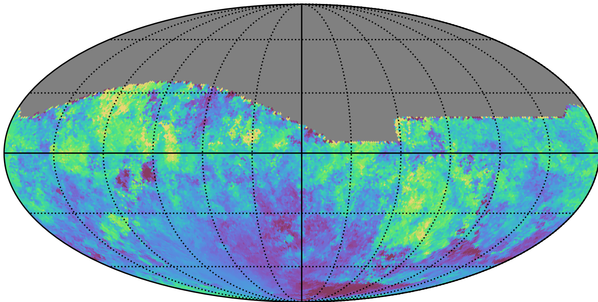
weather_cloudso14v3.4_10yrs All sky i band: Median moonDistance
