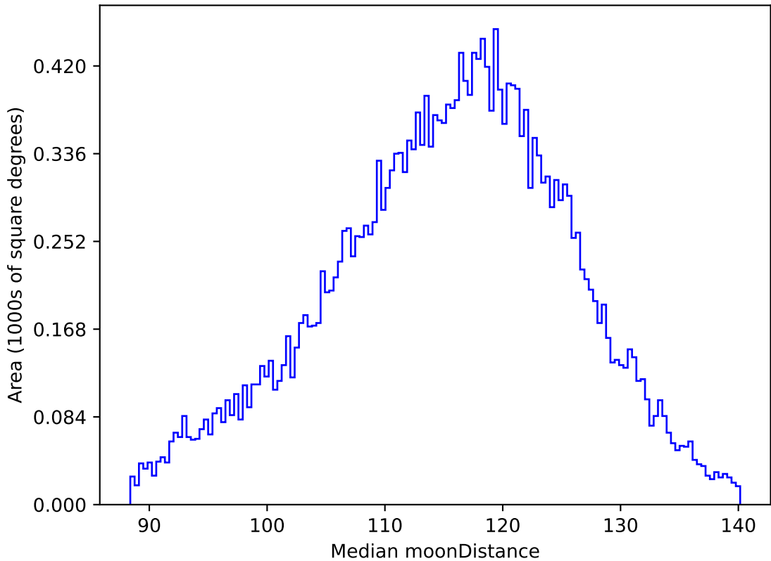
weather_cloudso14v3.4_10yrs All sky g band: Median moonDistance
