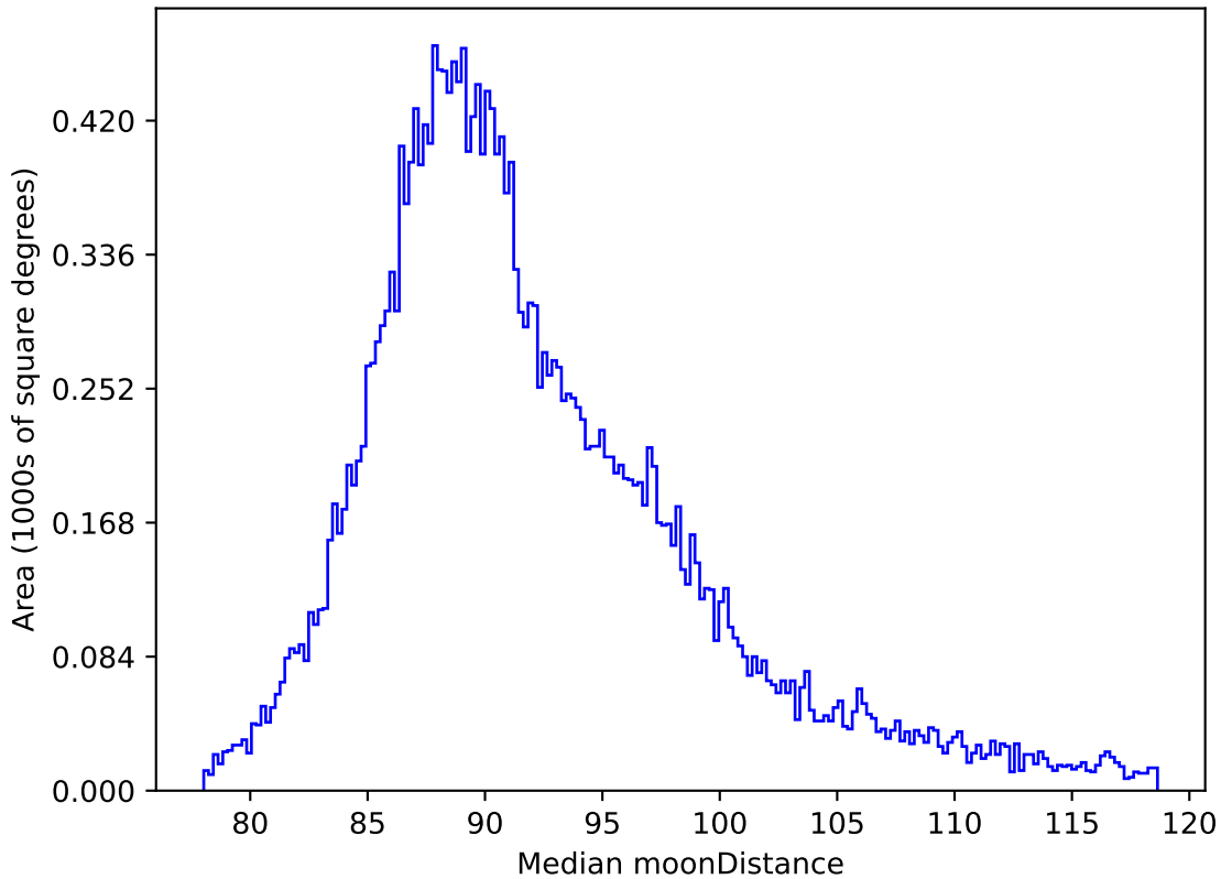
weather_cloudso14v3.4_10yrs All sky all bands: Median moonDistance
