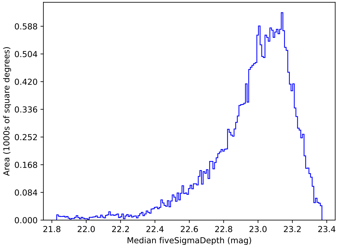
weather_cloudso14v3.4_10yrs Yr 1 z band: Median fiveSigmaDepth
