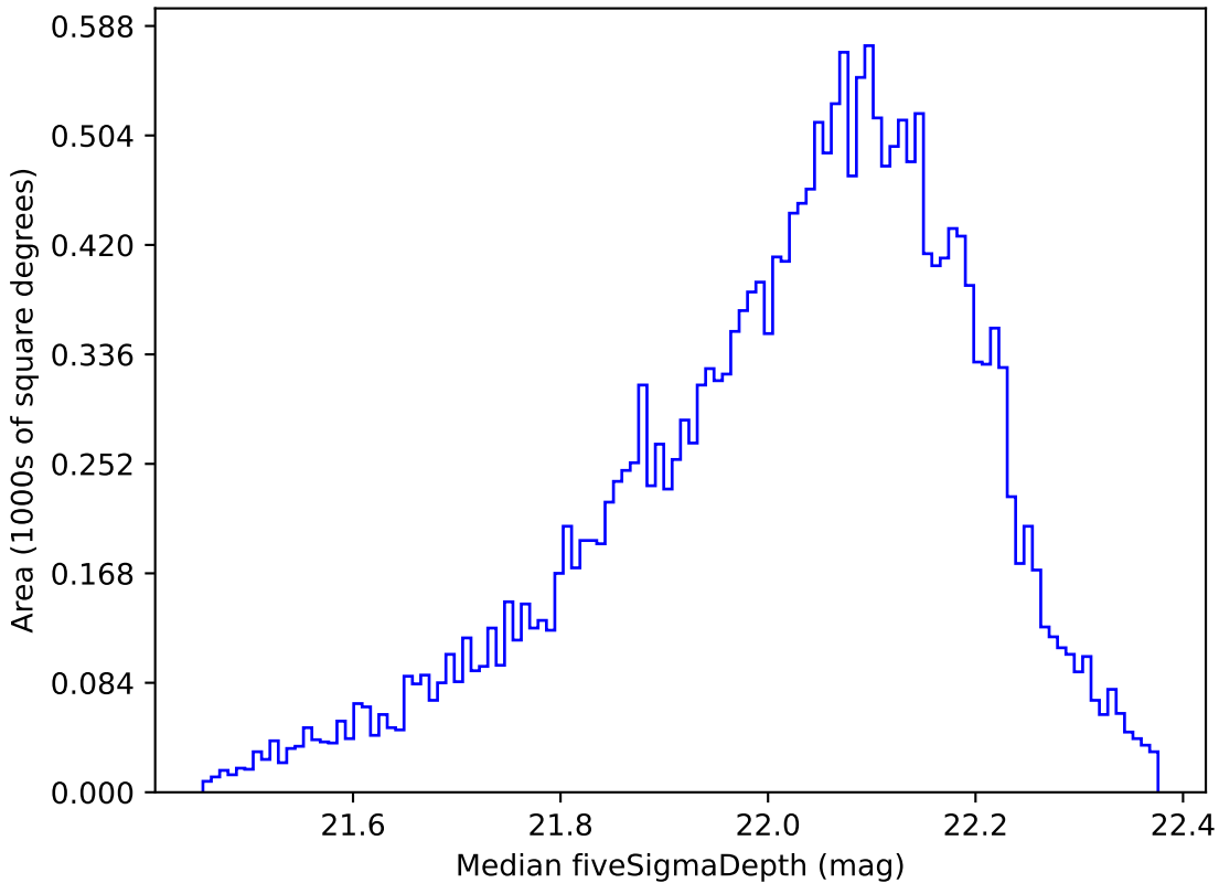
weather_cloudso14v3.4_10yrs Yr 1 y band: Median fiveSigmaDepth
