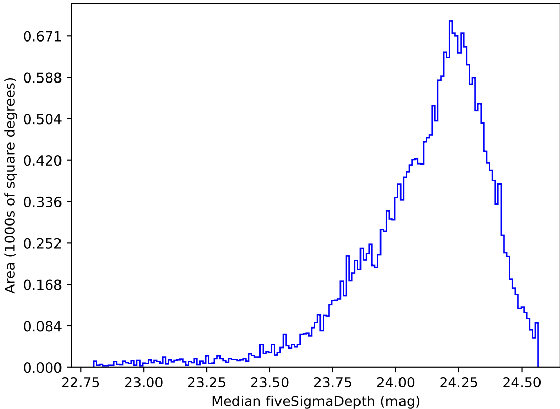
weather_cloudso14v3.4_10yrs Yr 1 r band: Median fiveSigmaDepth
