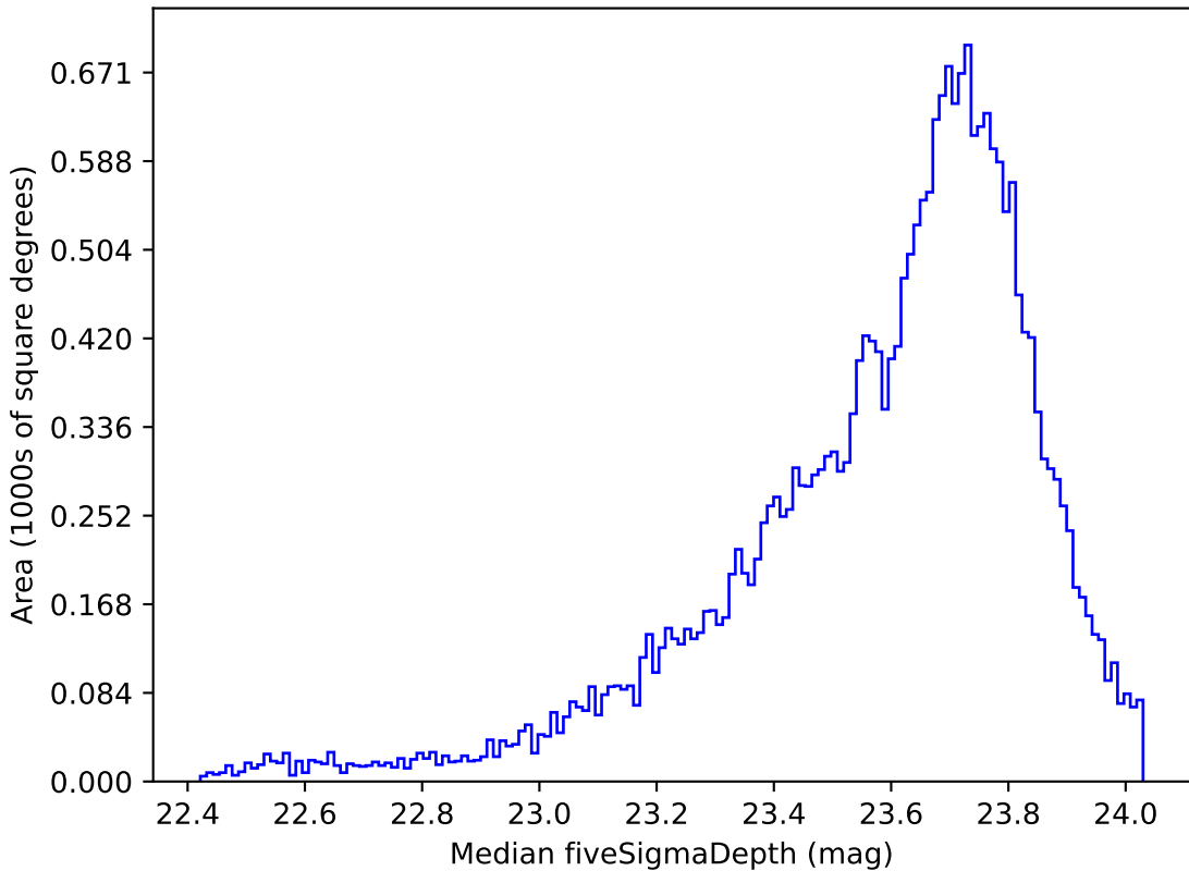
weather_cloudso14v3.4_10yrs Yr 1 i band: Median fiveSigmaDepth
