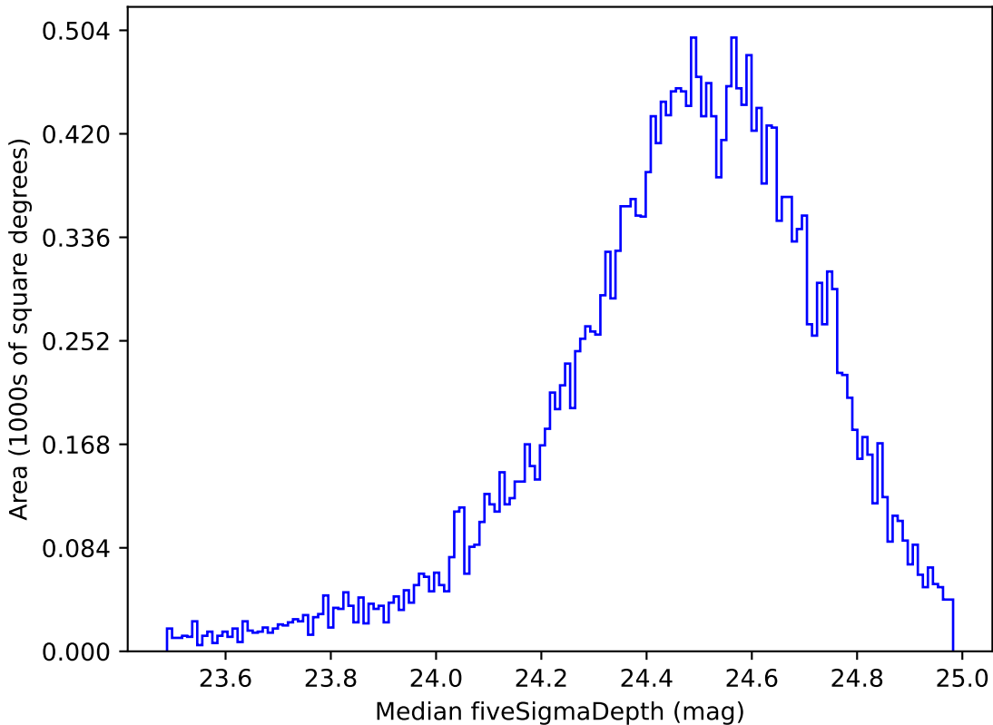
weather_cloudso14v3.4_10yrs Yr 1 g band: Median fiveSigmaDepth
