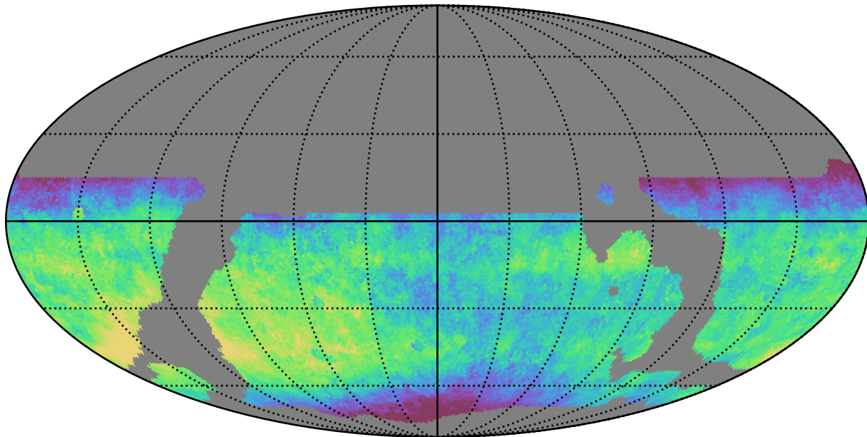
weather_cloudso14v3.4_10yrs WFD z band: Median fiveSigmaDepth
