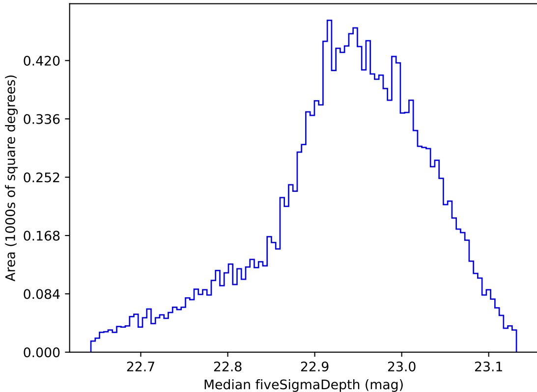
weather_cloudso14v3.4_10yrs WFD z band: Median fiveSigmaDepth
