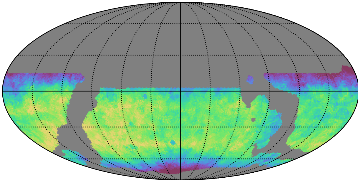
weather_cloudso14v3.4_10yrs WFD y band: Median fiveSigmaDepth
