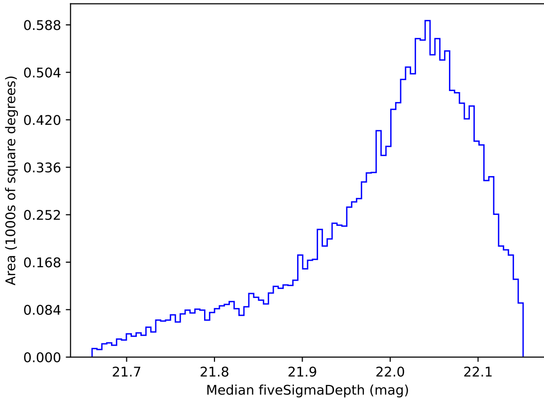
weather_cloudso14v3.4_10yrs WFD y band: Median fiveSigmaDepth
