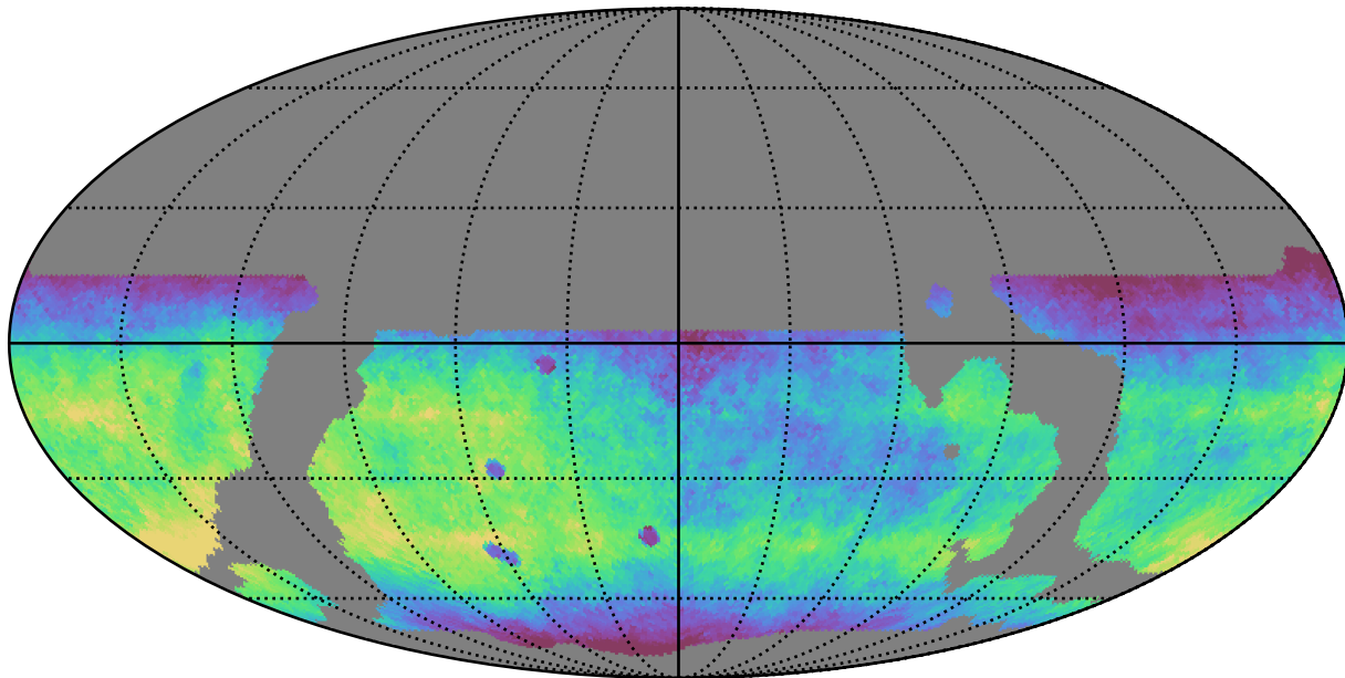
weather_cloudso14v3.4_10yrs WFD r band: Median fiveSigmaDepth
