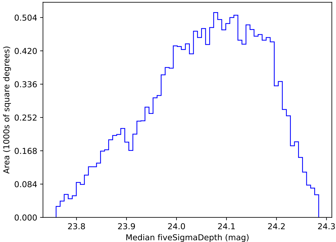
weather_cloudso14v3.4_10yrs WFD r band: Median fiveSigmaDepth
