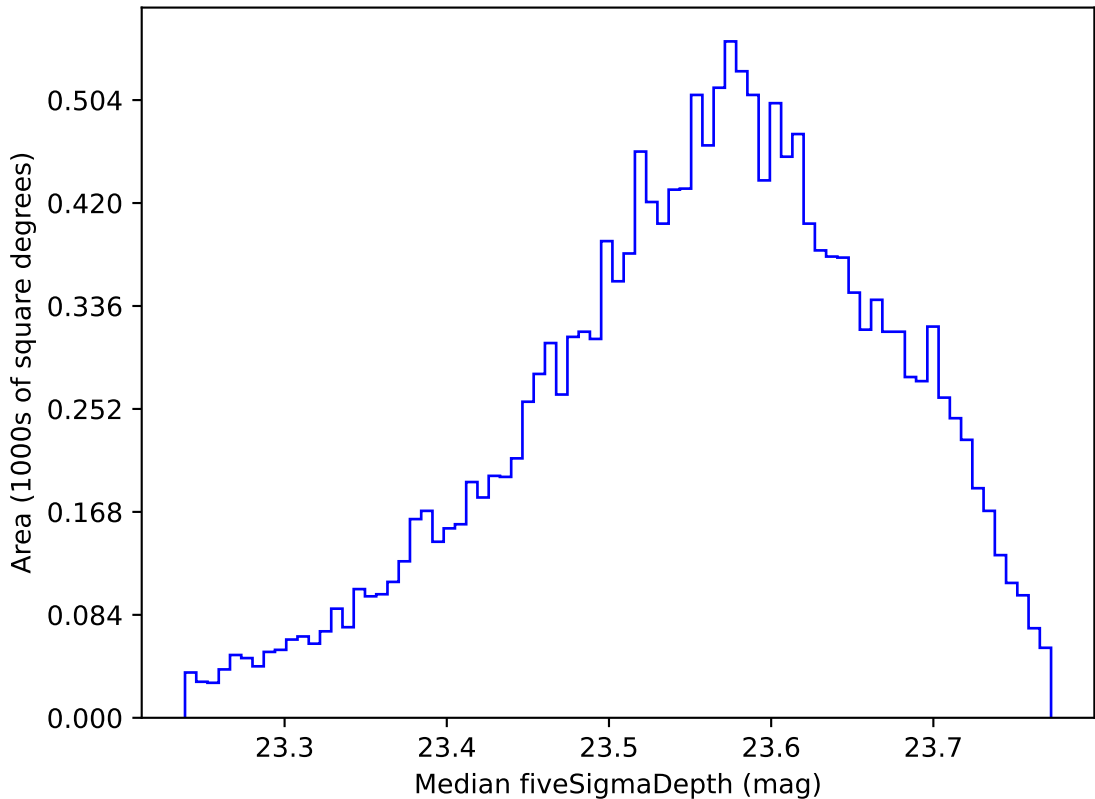
weather_cloudso14v3.4_10yrs WFD i band: Median fiveSigmaDepth
