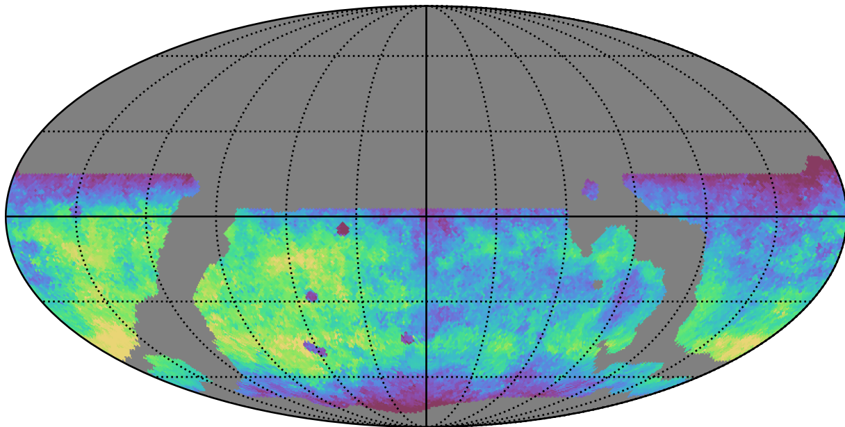
weather_cloudso14v3.4_10yrs WFD g band: Median fiveSigmaDepth
