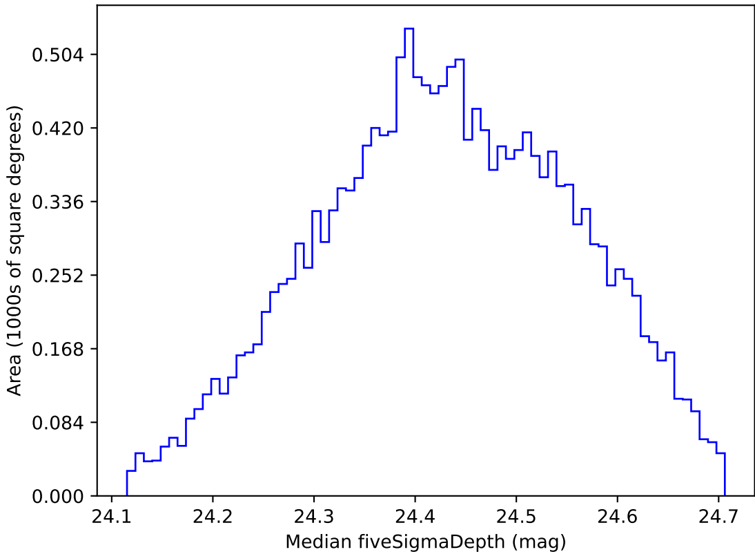
weather_cloudso14v3.4_10yrs WFD g band: Median fiveSigmaDepth
