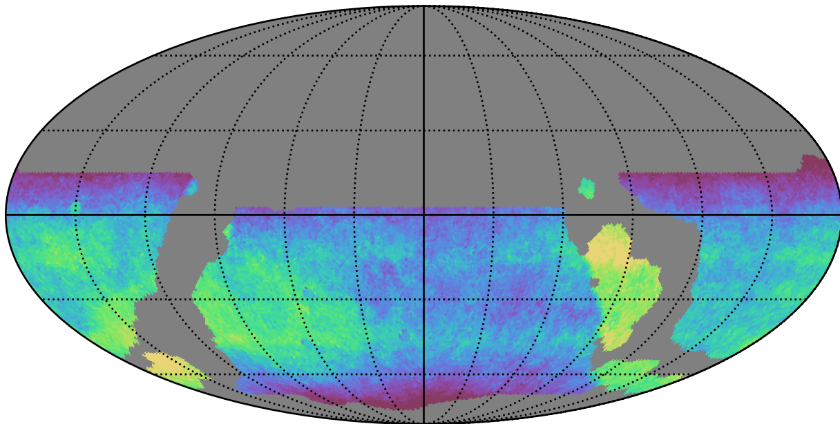
weather_cloudso14v3.4_10yrs WFD all bands: Median fiveSigmaDepth
