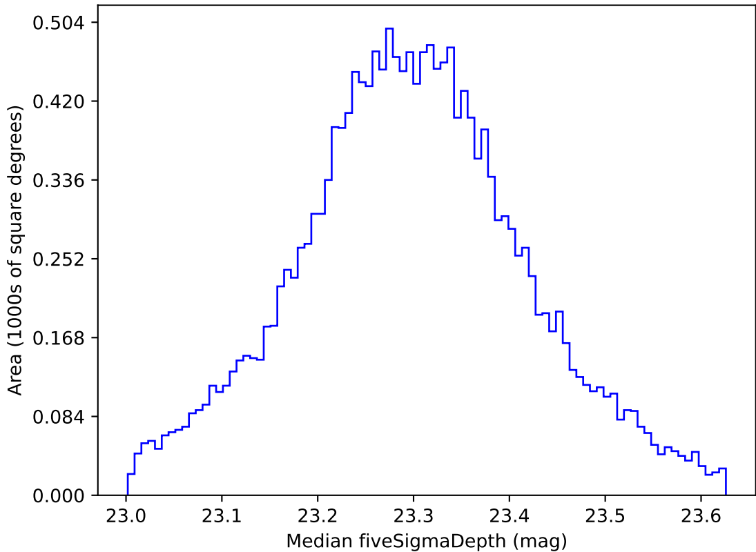
weather_cloudso14v3.4_10yrs WFD all bands: Median fiveSigmaDepth
