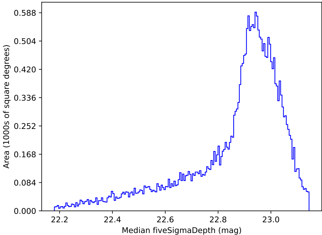
weather_cloudso14v3.4_10yrs All sky z band: Median fiveSigmaDepth
