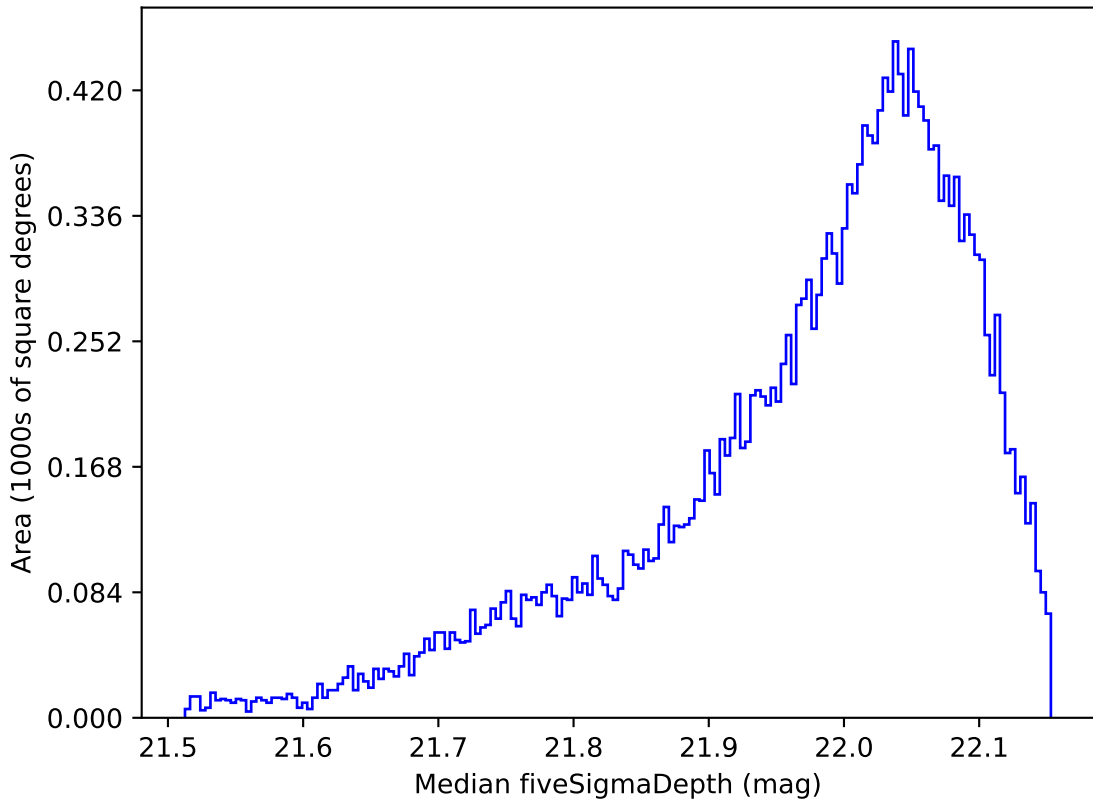
weather_cloudso14v3.4_10yrs All sky y band: Median fiveSigmaDepth
