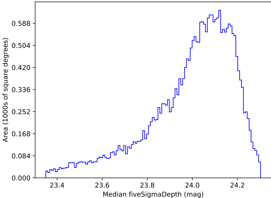
weather_cloudso14v3.4_10yrs All sky r band: Median fiveSigmaDepth
