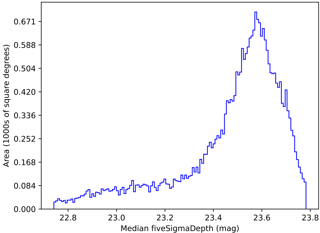
weather_cloudso14v3.4_10yrs All sky i band: Median fiveSigmaDepth
