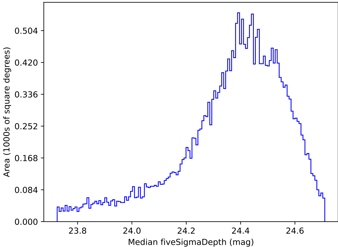
weather_cloudso14v3.4_10yrs All sky g band: Median fiveSigmaDepth
