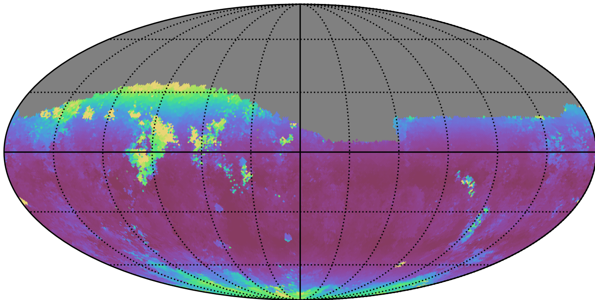
weather_cloudso14v3.4_10yrs Yr 1 z band: Median airmass
