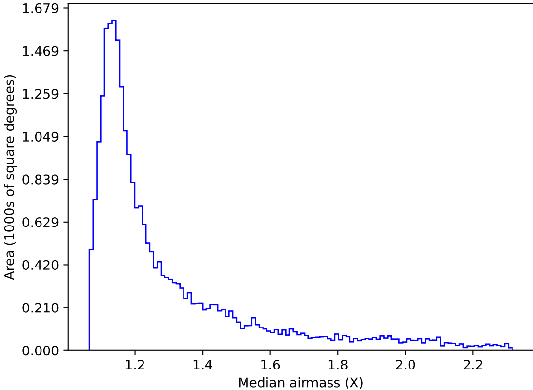
weather_cloudso14v3.4_10yrs Yr 1 z band: Median airmass
