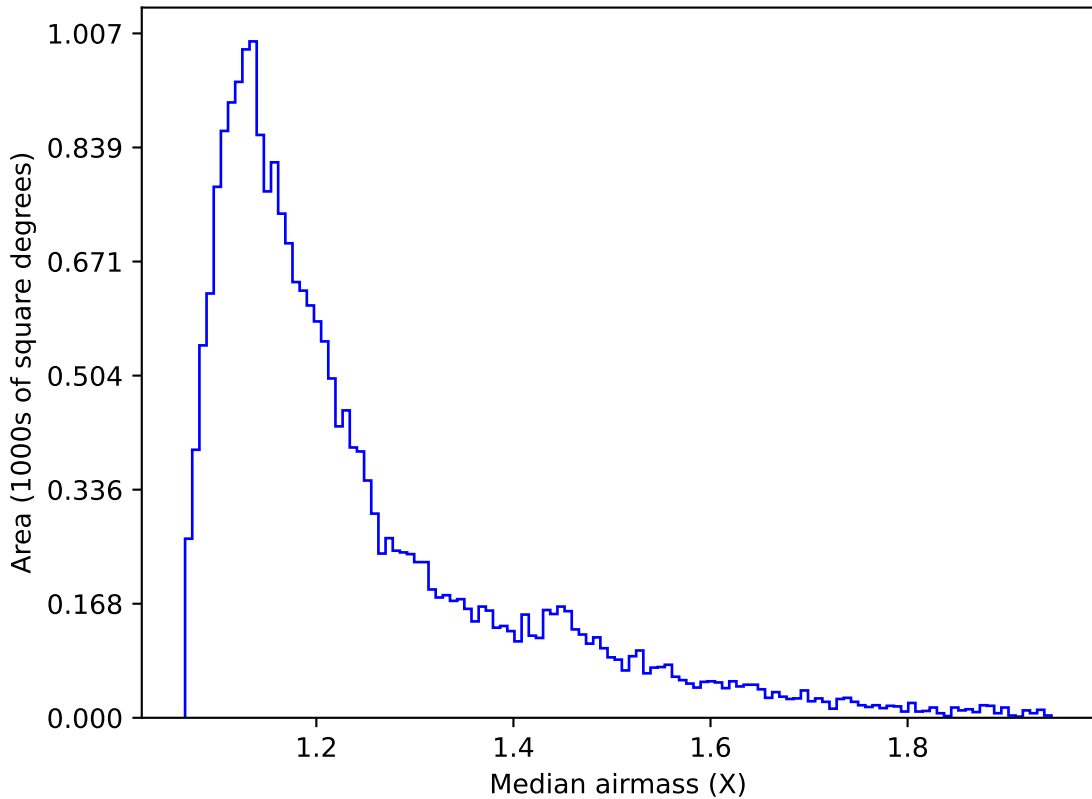
weather_cloudso14v3.4_10yrs Yr 1 y band: Median airmass
