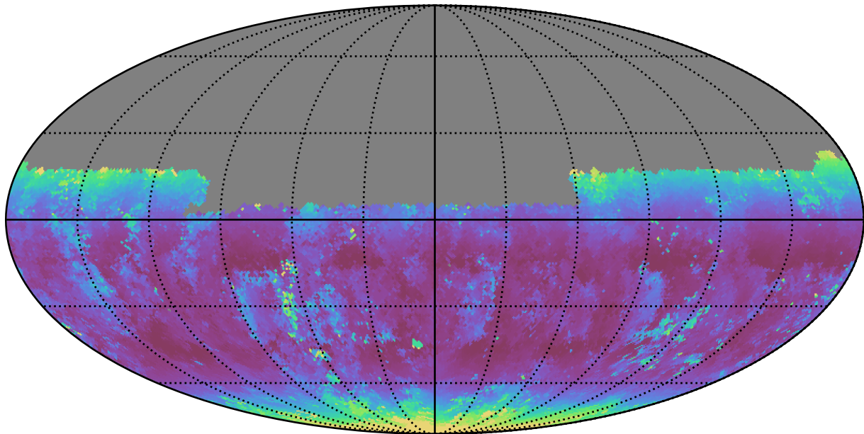
weather_cloudso14v3.4_10yrs Yr 1 u band: Median airmass
