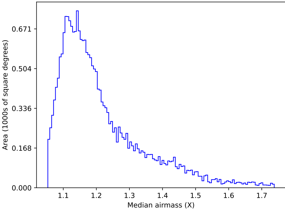
weather_cloudso14v3.4_10yrs Yr 1 u band: Median airmass
