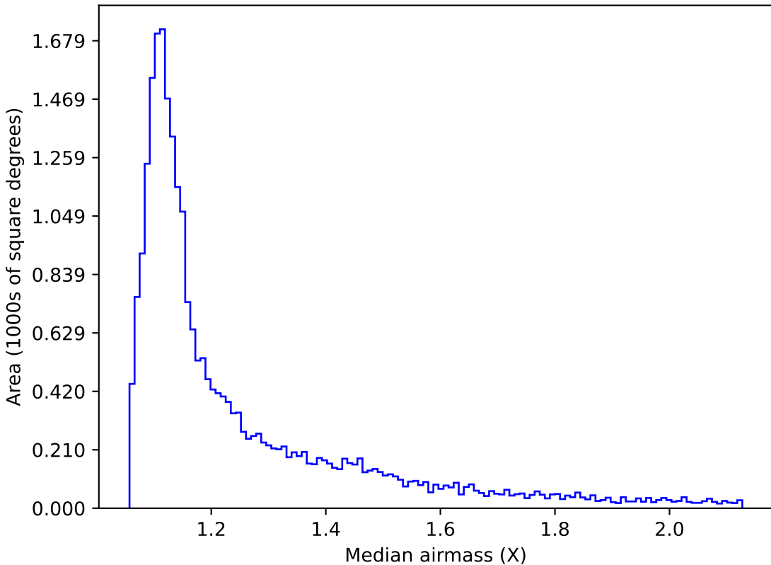
weather_cloudso14v3.4_10yrs Yr 1 r band: Median airmass
