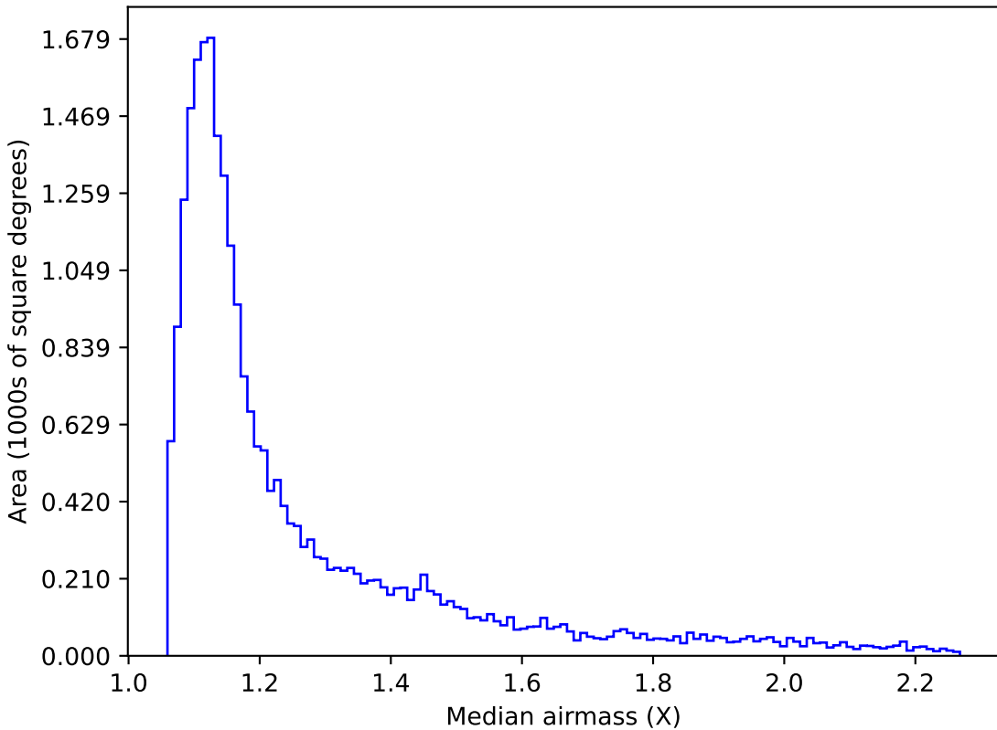
weather_cloudso14v3.4_10yrs Yr 1 i band: Median airmass
