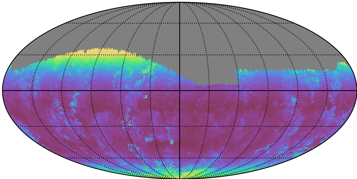
weather_cloudso14v3.4_10yrs Yr 1 g band: Median airmass
