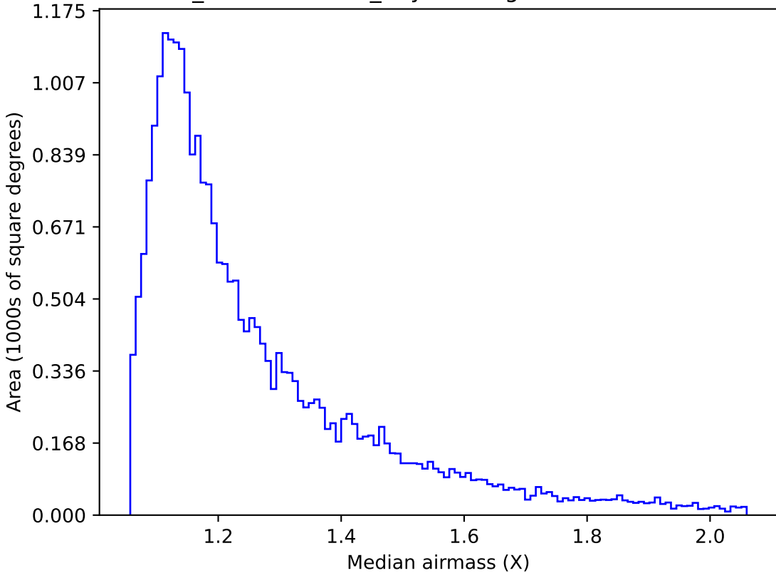
weather_cloudso14v3.4_10yrs Yr 1 g band: Median airmass
