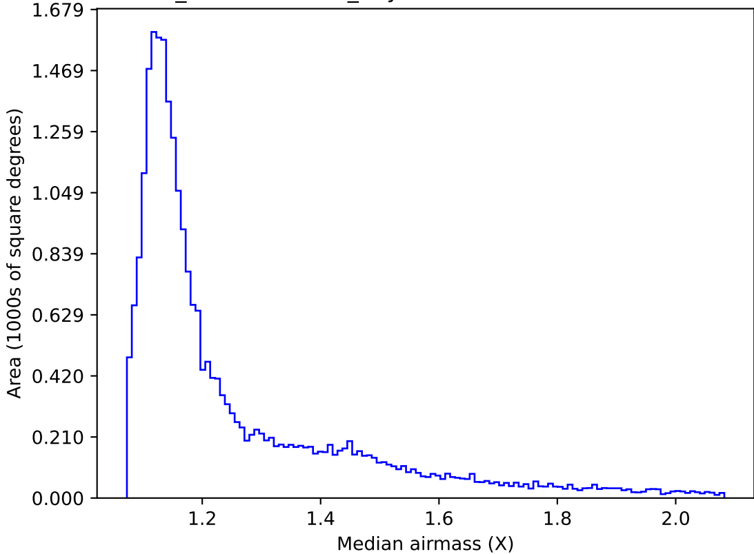
weather_cloudso14v3.4_10yrs Yr 1 all bands: Median airmass
