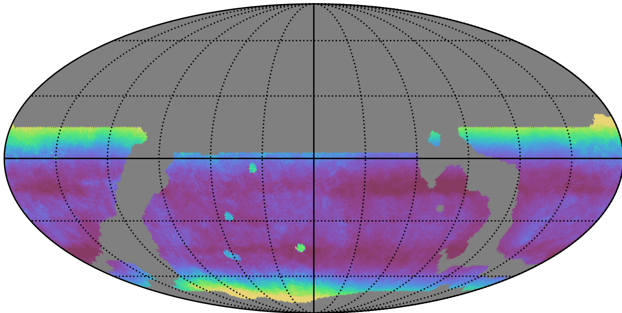
weather_cloudso14v3.4_10yrs WFD z band: Median airmass
