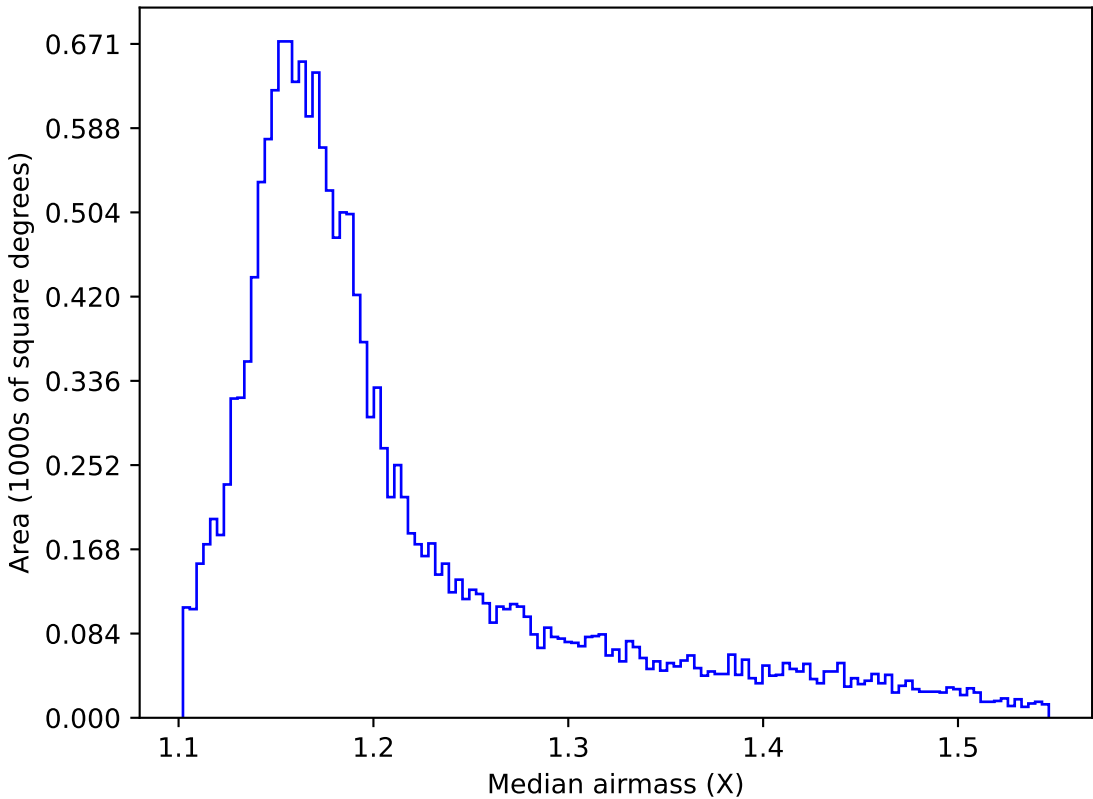
weather_cloudso14v3.4_10yrs WFD y band: Median airmass
