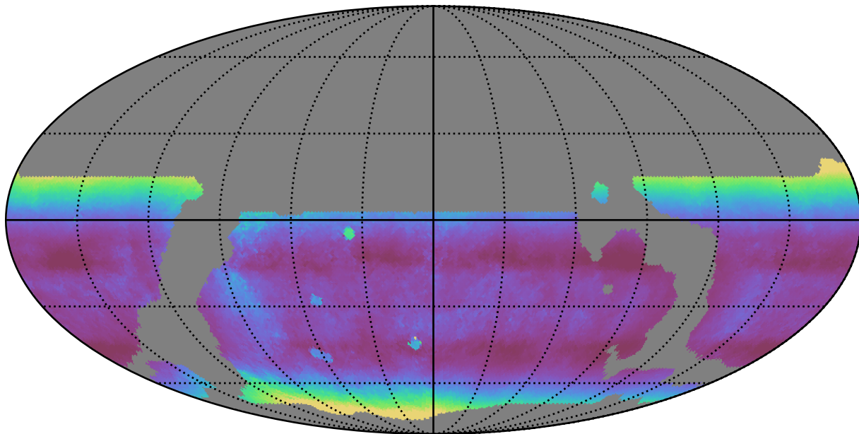
weather_cloudso14v3.4_10yrs WFD r band: Median airmass
