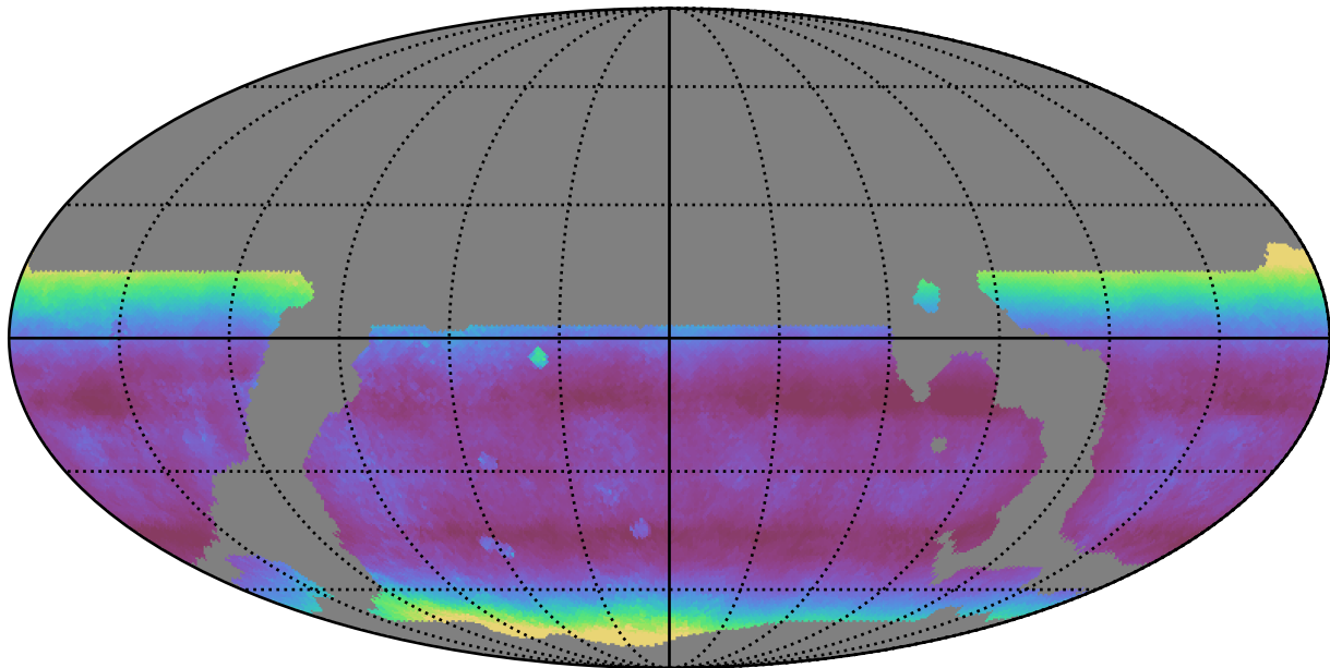
weather_cloudso14v3.4_10yrs WFD i band: Median airmass
