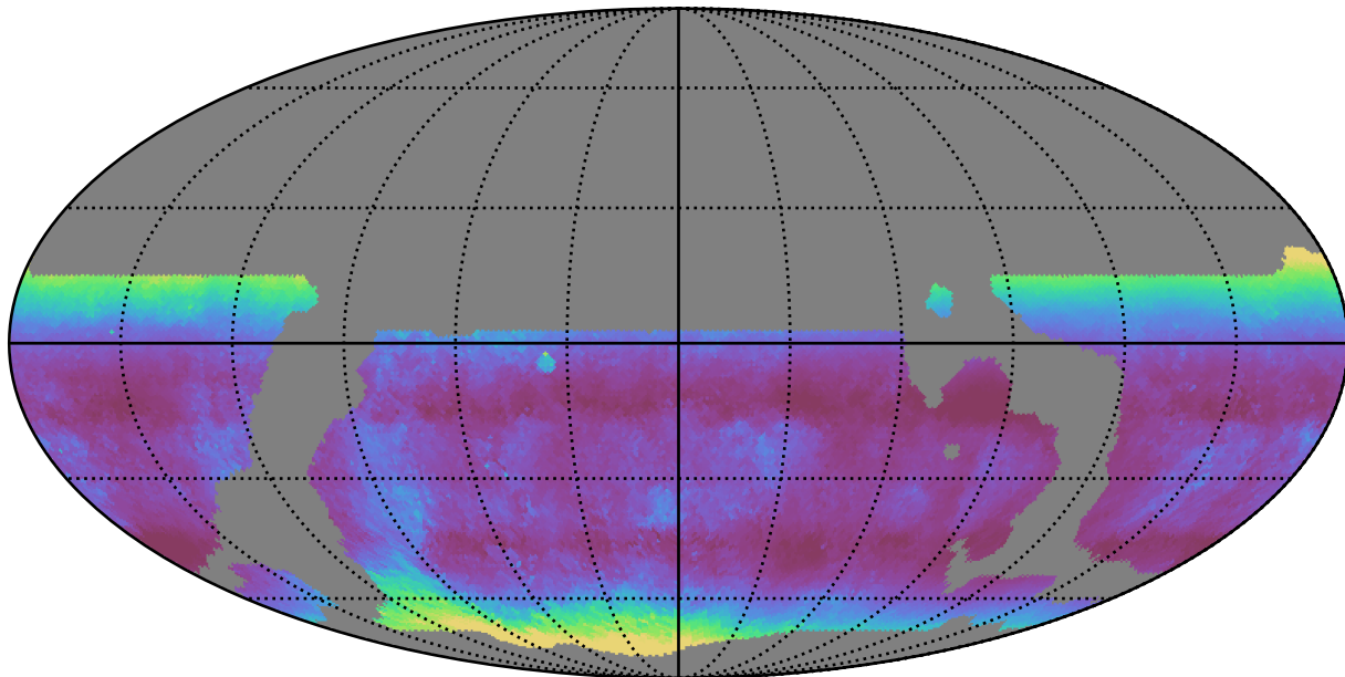
weather_cloudso14v3.4_10yrs WFD g band: Median airmass
