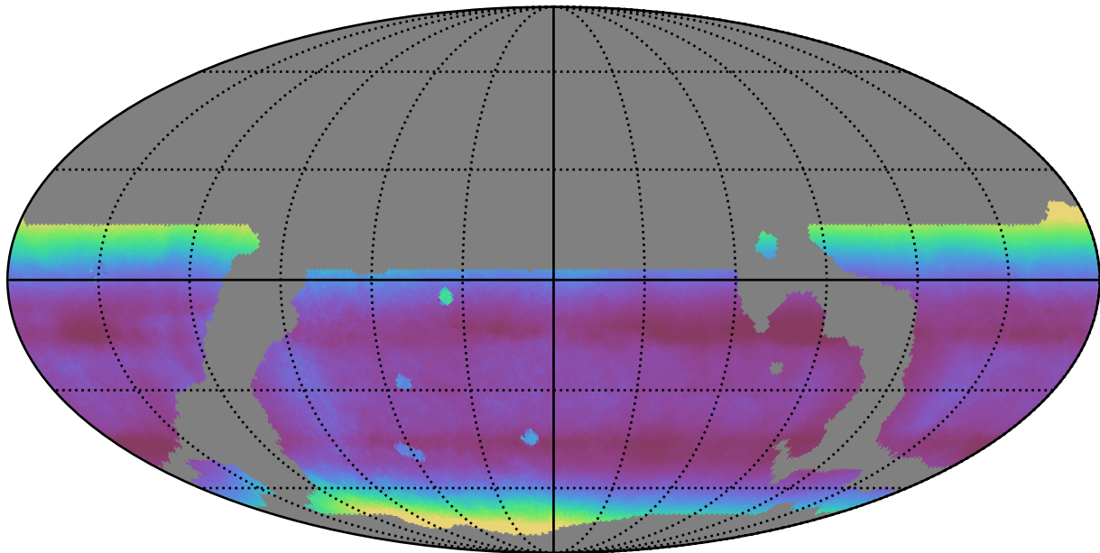
weather_cloudso14v3.4_10yrs WFD all bands: Median airmass
