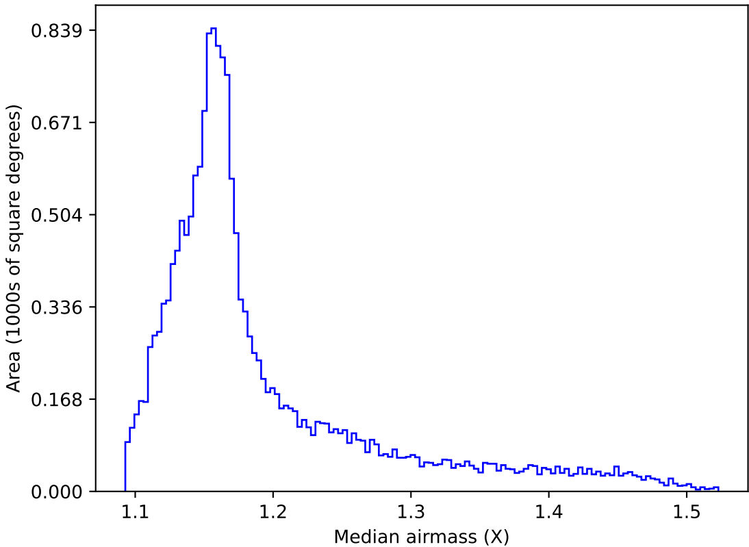
weather_cloudso14v3.4_10yrs WFD all bands: Median airmass
