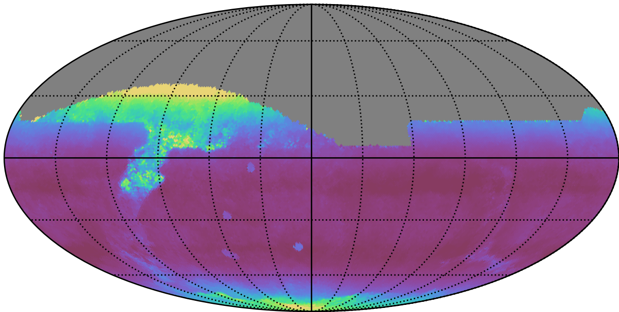
weather_cloudso14v3.4_10yrs All sky z band: Median airmass
