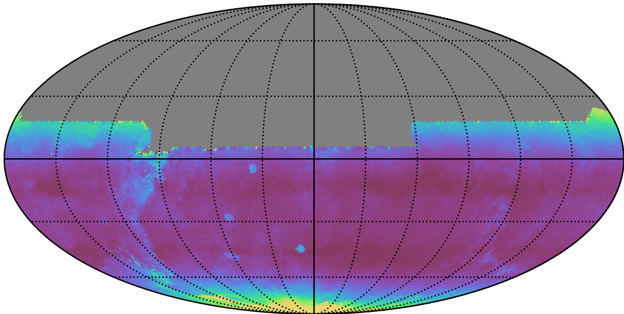
weather_cloudso14v3.4_10yrs All sky y band: Median airmass
