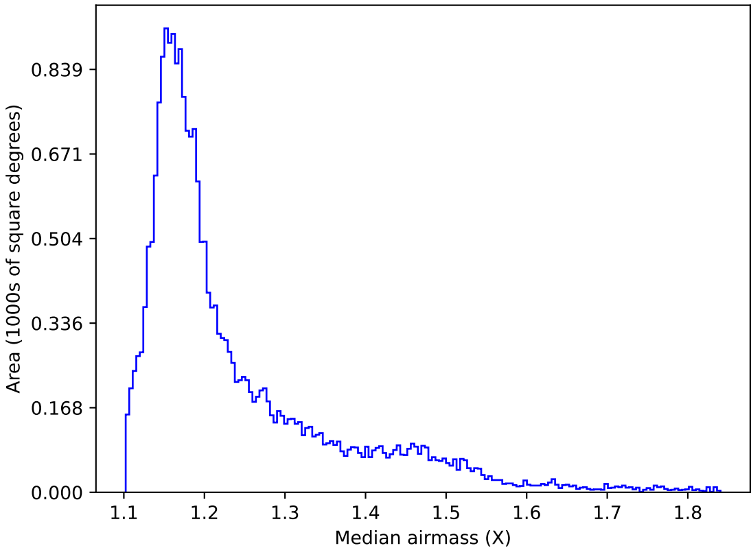
weather_cloudso14v3.4_10yrs All sky y band: Median airmass
