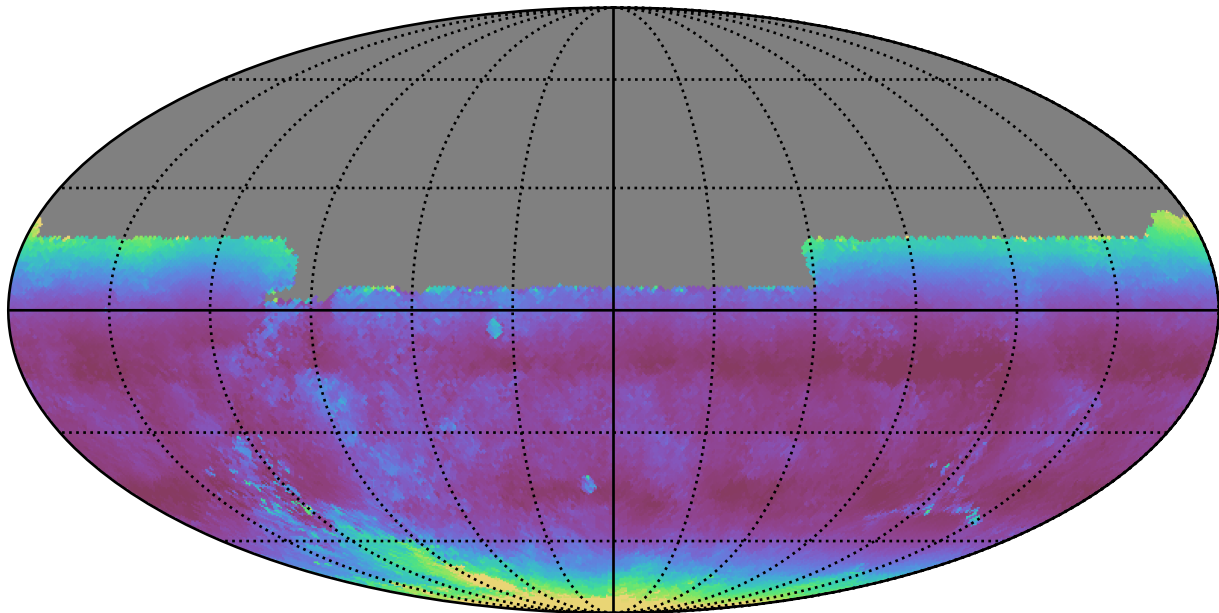
weather_cloudso14v3.4_10yrs All sky u band: Median airmass
