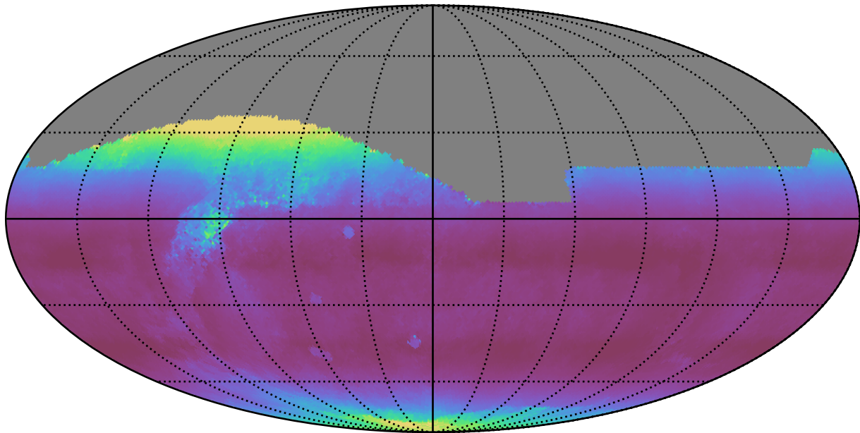
weather_cloudso14v3.4_10yrs All sky r band: Median airmass
