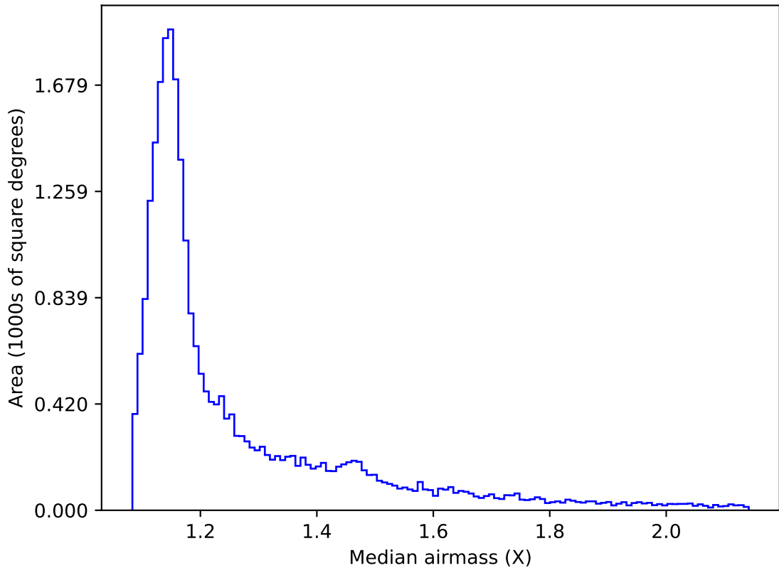
weather_cloudso14v3.4_10yrs All sky r band: Median airmass
